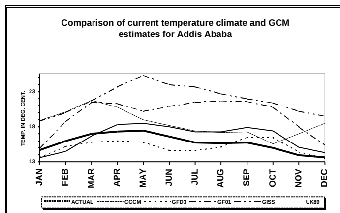
Figure 5.7: Selected Temperature Validation Results of GCMs at Addis Ababa (from Ademe and Kinfu, 2000)
