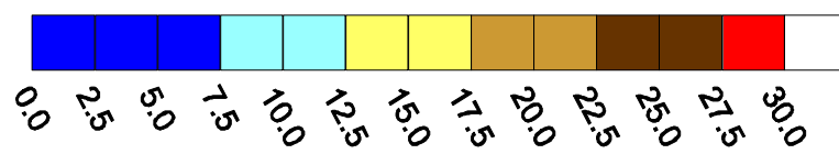
Figure 2.7: Daily Minimum Temperature for the Year (°C)
