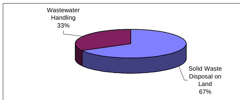
Figure 3.6: Percentage Contributions of Methane Emissions from Solid Waste Disposal on Land from Addis Ababa City and Other Urban Centers and Wastewater Handling in 1994.
